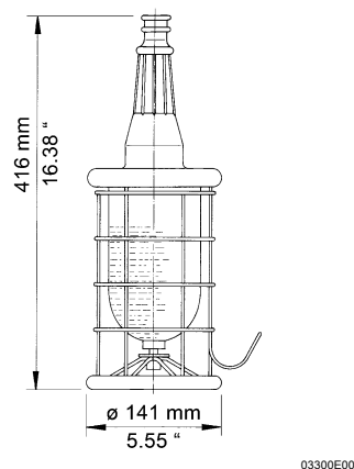
Hand lamp, 6147
