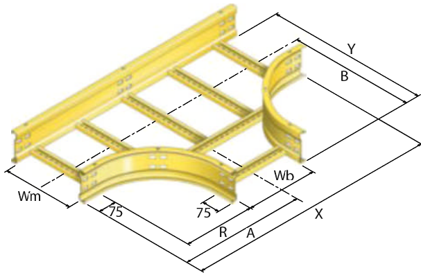
Speedway 750mm Radius Tees
