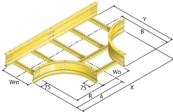
Speedway 1050mm Radius Tees
