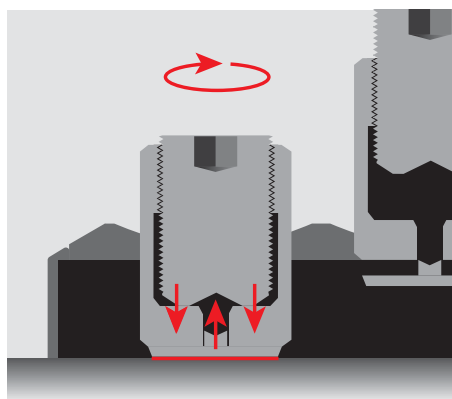
As the SICON bolt is screwed in, the friction disc at the base of the bolt breaks away. The bolt now turns on this disc; unlike with conventional bolts, no tip friction occurs on the conductor
