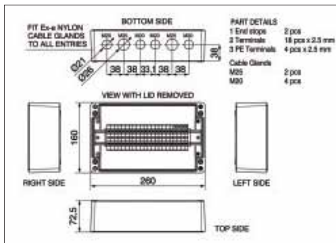
Terminal Box Assembly Drawing
