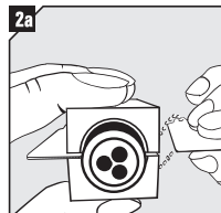
Measure the gap with the Ex Gap Gauge by holding blade one in one gap and checking the other with blade two.
