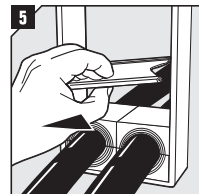
Insert a stayplate on top of every finished row of modules.
