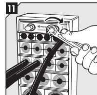
Tighten the screws until full stop, approx 20 Nm (15 ft.lb.).
