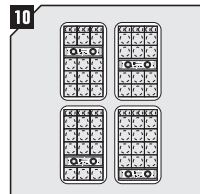
The Roxtec Wedge Ex can be placed anywhere in the frame.
