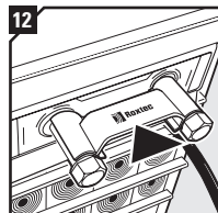
Attach the Wedge Clip to the wedge bolts to check that the wedge has been properly tightened.
