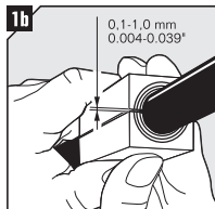
Achieve a 0.1-1.0 mm gap between the two halves when held against the cable/pipe. Use the Ex Gap Gauge.
