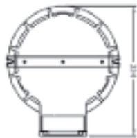
621 Bulkhead
