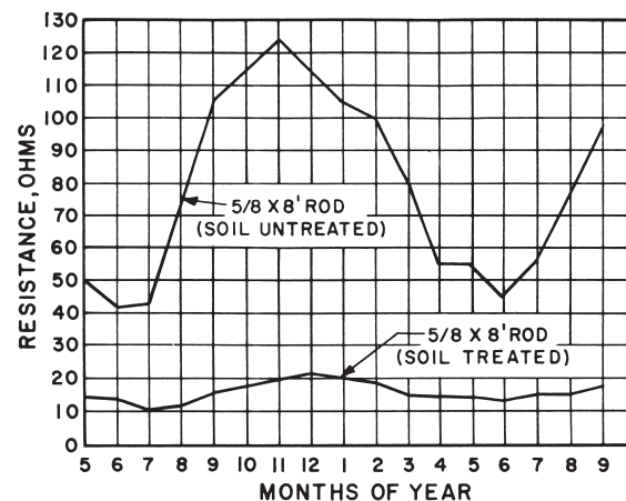
Fig. 15: Chemical treatment of soil lessens seasonal variation of electrodes' earth resistance 8
