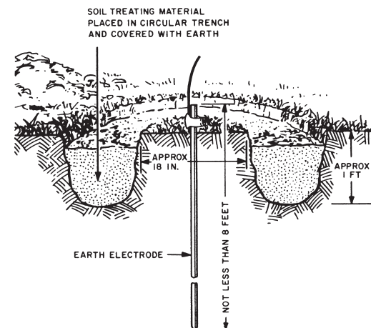
Fig. 14: Trench method of soil treatment 7
