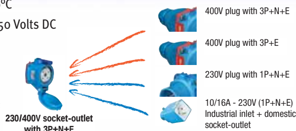
Coupler socket
