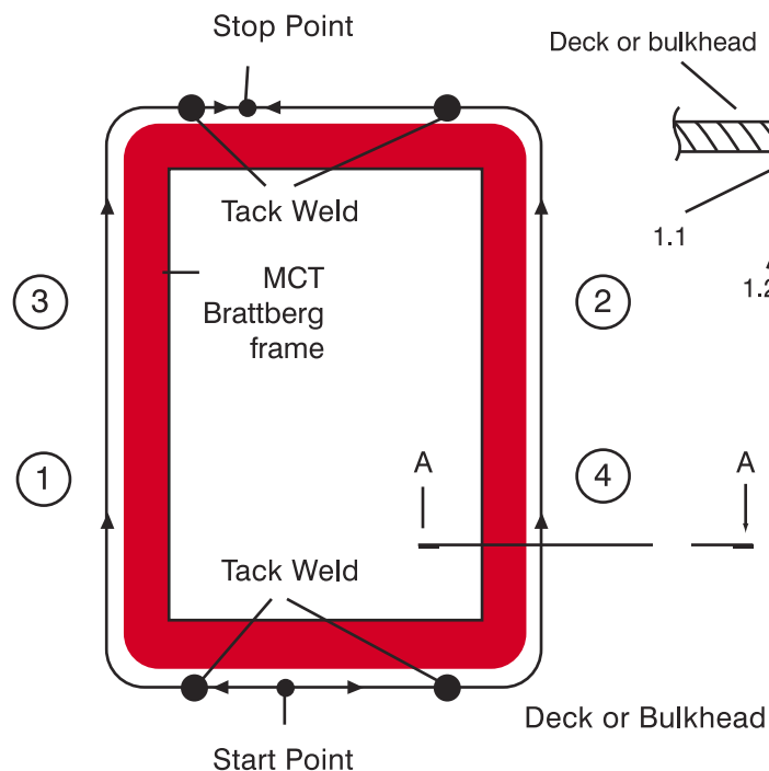
FIG 4: Welding sequence
