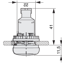
Pilot Light, Flush, for BA9s Bulb
