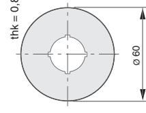
Emergency Stop Plate P SN/XBK1
