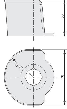
Protective Shroud
