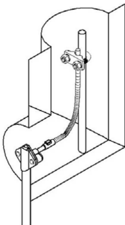
TYPICAL EBP2P-T
