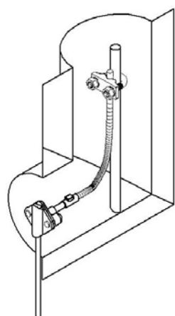
TYPICAL EBP2P-08-T
