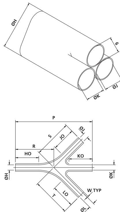
573H532-535 series as supplied / recovered.
