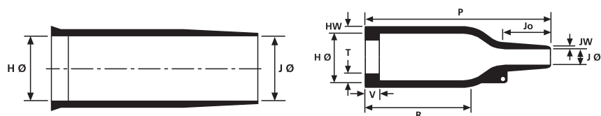
Recovered 199-4-G, VG style shape for small audio connectors with external ribs for improved grip.
