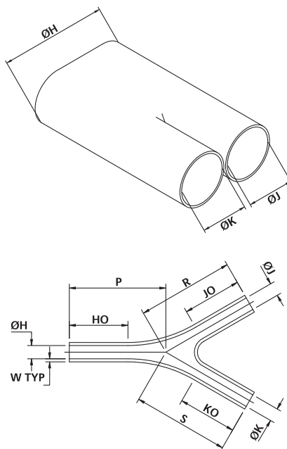
492H412-415 series as supplied / recovered.
