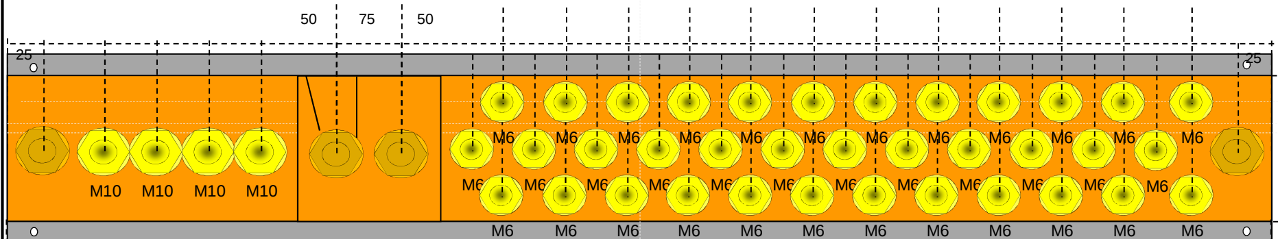
BRASS ASSEMBLY
