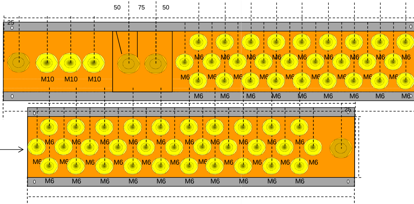
INSULATOR
