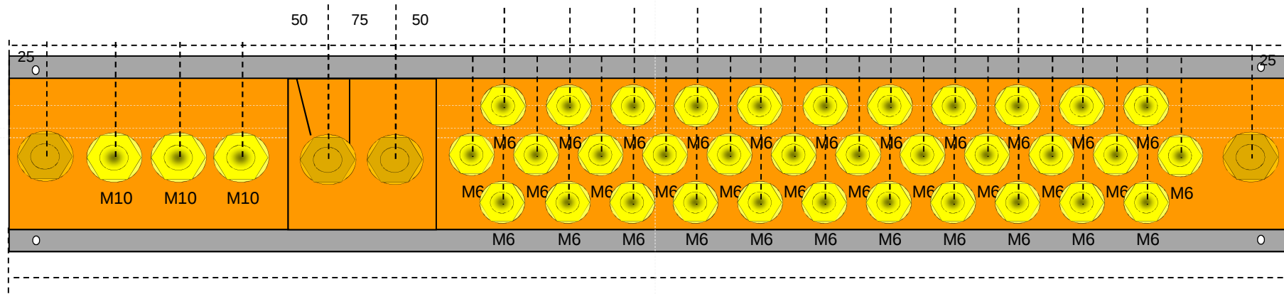
BRASS ASSEMBLY
