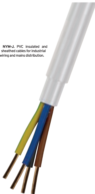
6491 X. PVC insulated single cores for installation in cable management systems.
