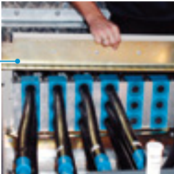
Openable frames for easier installation of power cables in cabinets.
