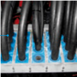
Retention systems below nacelle and in tower.
