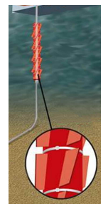
> Strakes
