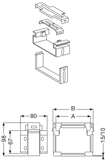
IP44 joint
