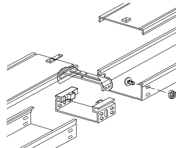
Integral mechanical joint
