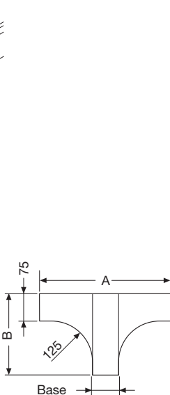
Vertical tee
