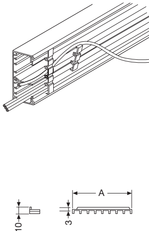
Cable retainer
