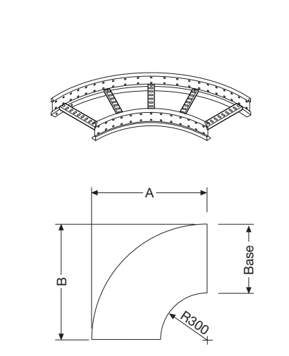
90° flat corner
