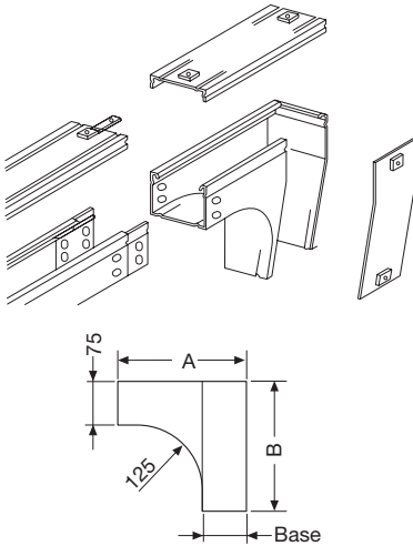
Left 90° outside riser
