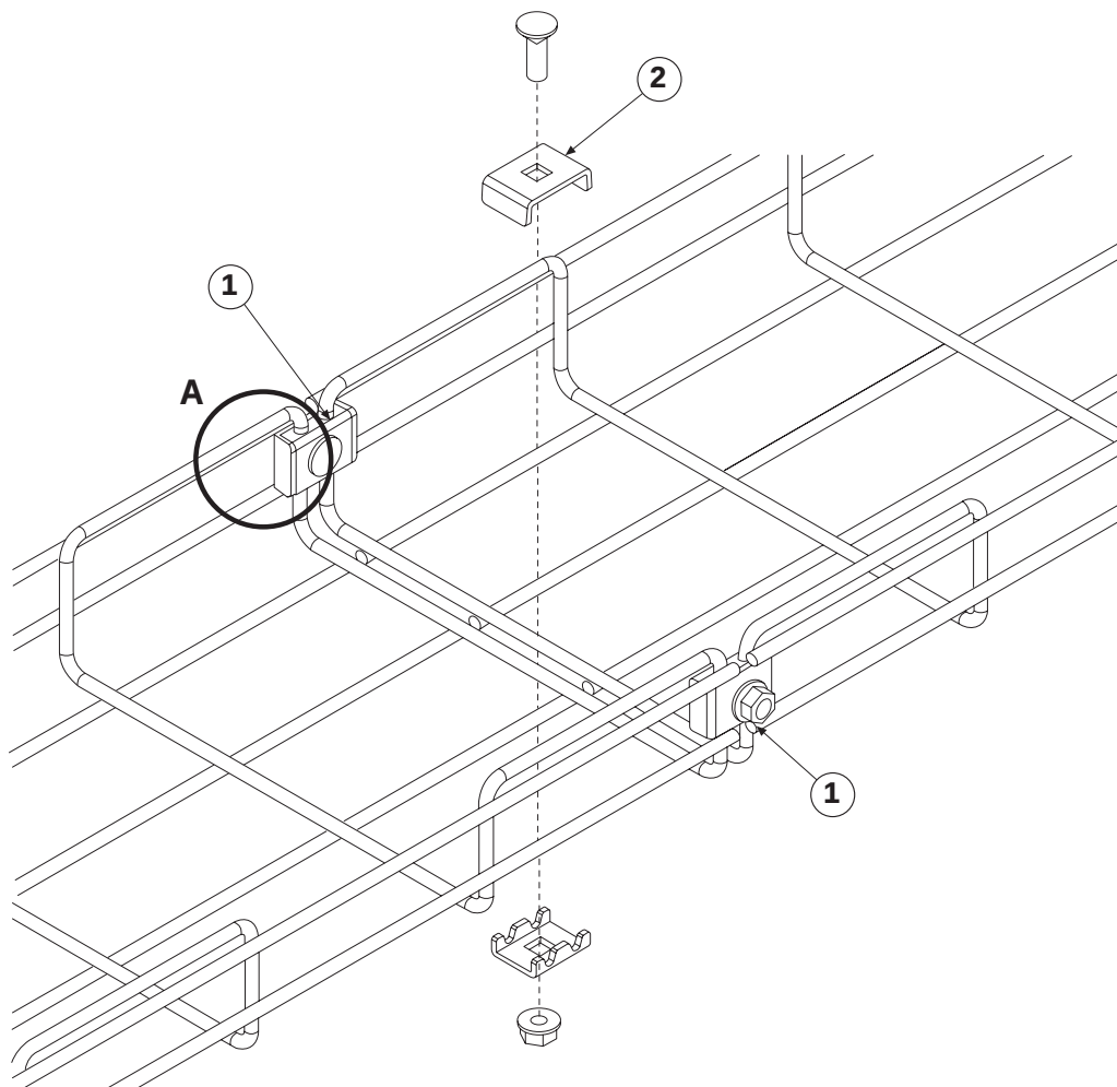
Detail A
