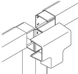
Tee branch
