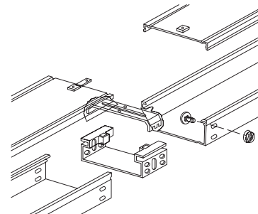
Integral mechanical joint
