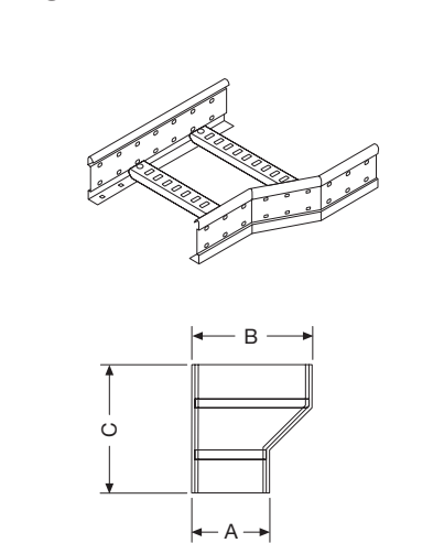
Right reducer
