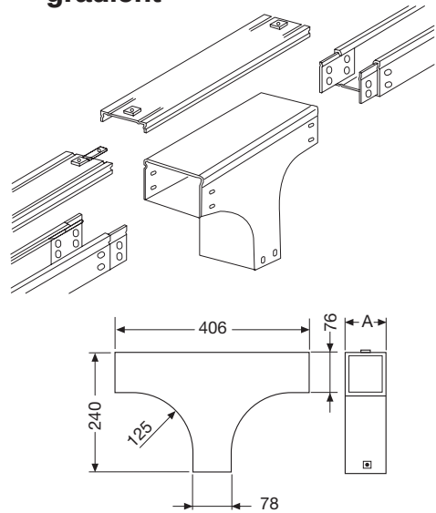
Vertical tee without level gradient
