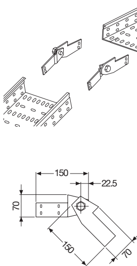
Adjustable joint
