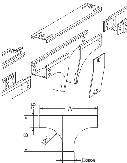
Vertical tee with level gradient
