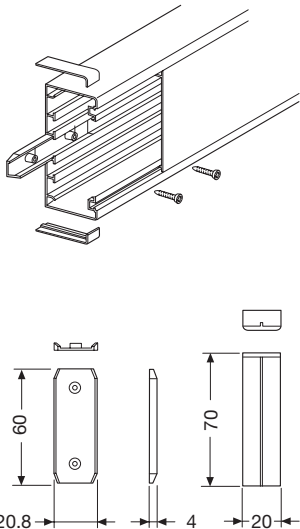
Flat joint for trunkings
