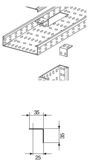
Vertical joint fixed at 90°
