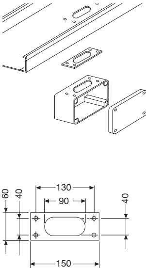
Branch connection coupler
