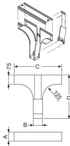
Vertical tee with reduction
