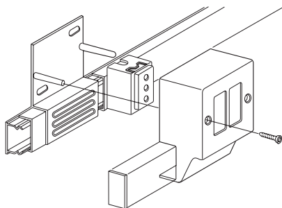
Switch-socket floor box (2 devices)
