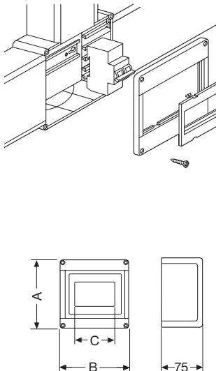
Consumer unit for 17.5x45 mm MCBs
