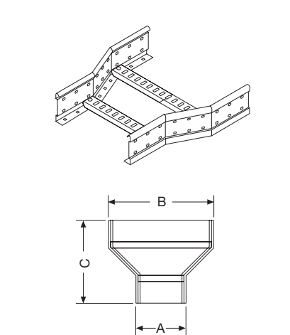
Concentric reducer
