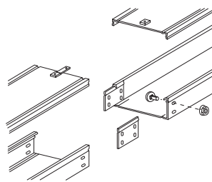
Mechanical joint for trunkings
