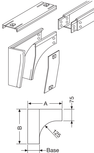
Right 90° outside riser
