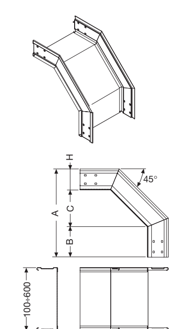
90° vertical outside riser
