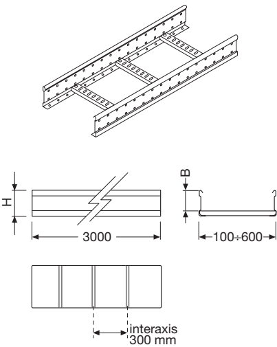
Cable ladder
