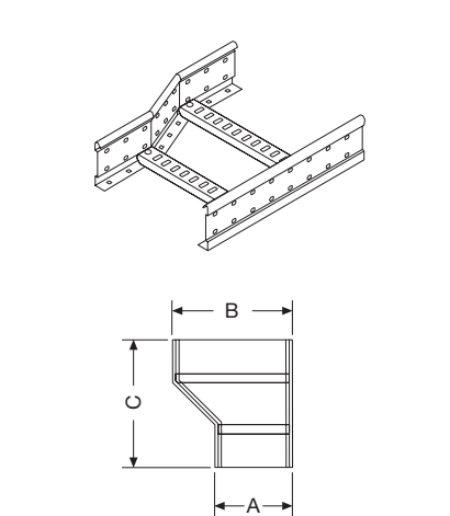
Left reducer
