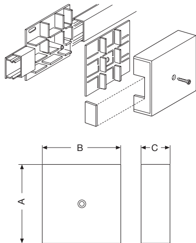
Box for flat branch connections
