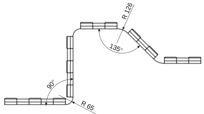
Cable tray H 50 mm
