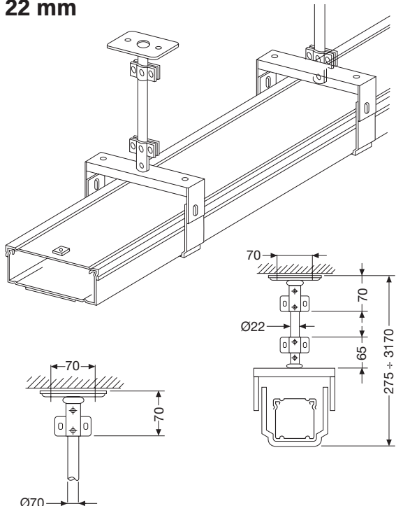
Plate with conduit-tightening collar Ø 22 mm
