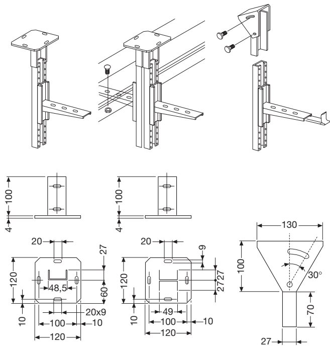
Ceiling anchorage plate
