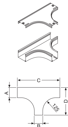
Flat tee with reduction
