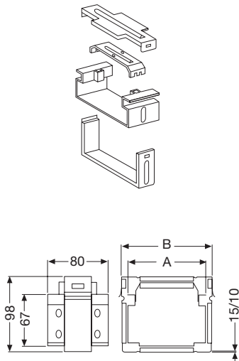
IP44 joint
