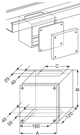
Metal branch connection box IP55
