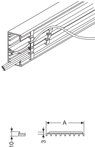
Cable retainer
