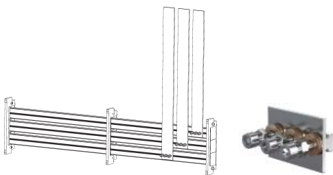
Example of connection at the rear. AB 2500 CSS
