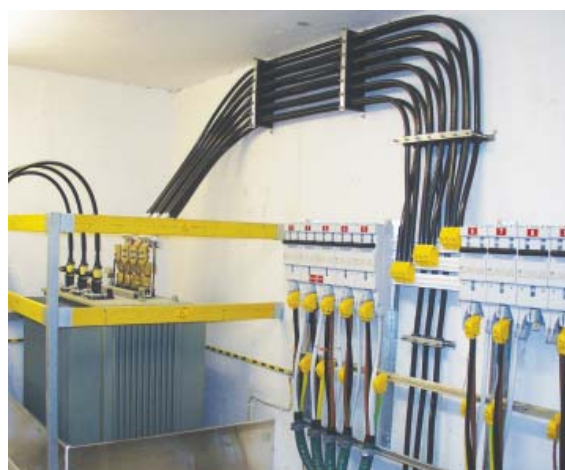
Kabeldon low voltage products mounted directly on a wall in a substation in Trondheim, Norway.
