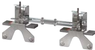
ILM 250 Interlocking mechanism for SEKOD 250.
