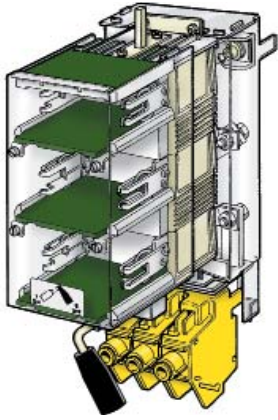
SEKO 160 Switch-fuse with breaking on both sides of the fuse.
