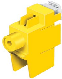
AD 2150 Insulated connector for parallel conductors.
