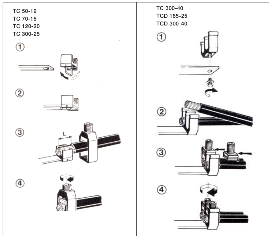
TC 300-40 Connecting clamps TC 300-40.
