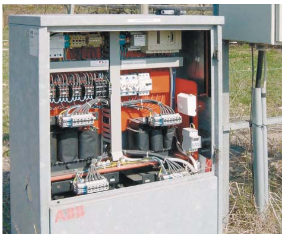
Kabeldon enclosure used for control equipment for adjustment of roundabout illumination at the entrance to Kalmar (E22), Sweden.
