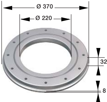
AFT 1703 Adapter flange for welding between APEGA 170 and transformer box.
