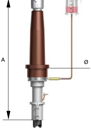
Dimension drawing for APEGA 84-170 kV.
