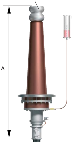
Dimension drawing for APEGA 245-420 kV.
