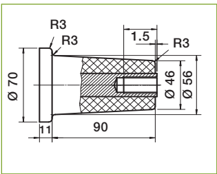
Standard bushing EN 50181 400 series, 630 A Contact type: Bolt M16 Interface type: C
