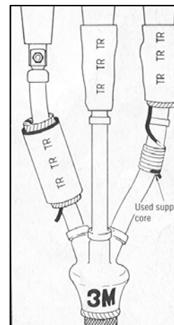
In-Line Barrier Boot System MB63
