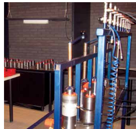
In-house fire testing and pressure testing at CSD International's Laboratories.
