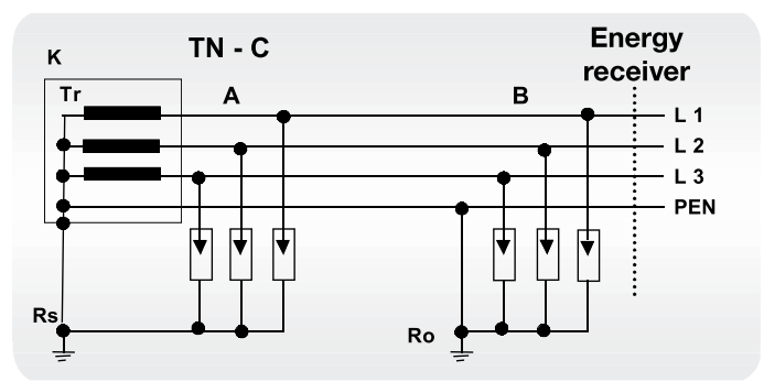
b) TN-C neutral and earthing conductor are common (PEN) and earthed at the transformer or near it
