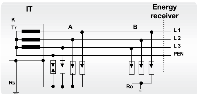
e) IT in this system there is no direct connection of active network parts with earth, while accessible conducting parts of installation elements are earthed
