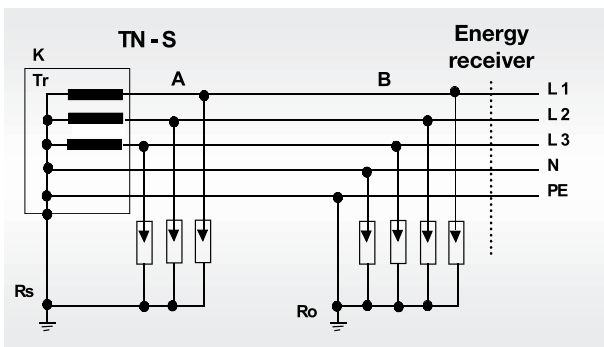
a) TN-S the supply network has a connection of the neutral conductor with the earthing conductor at the feeding transformer only
