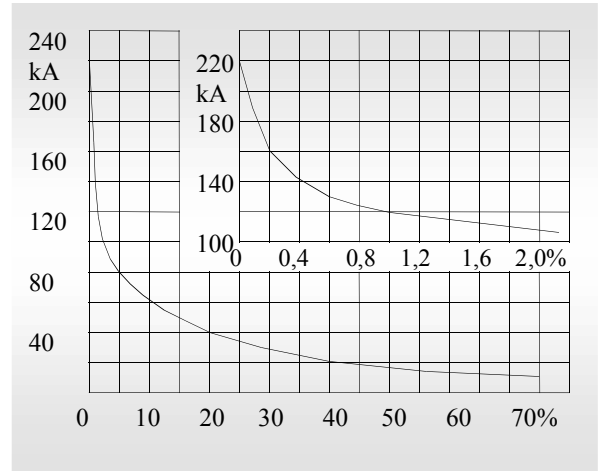
Figure. Lightning current occurrence probability of amplitude greater than values on axis of ordinates
