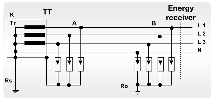
d) TT neutral point of transformer is earthed directly, while the receiver's installation is earthed by a separate earth electrode
