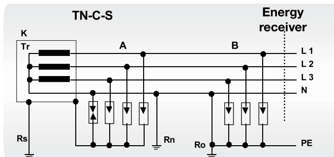
c) TN-C-S the neutral conductor is earthed at the transformer and in other network points
