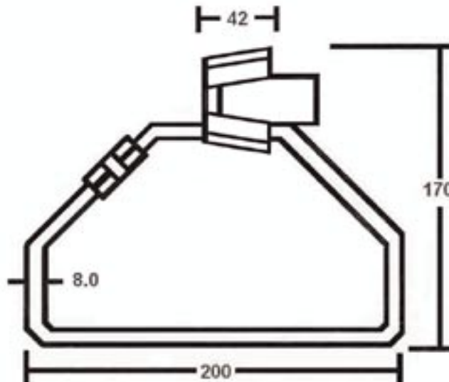
COPPER BAIL
