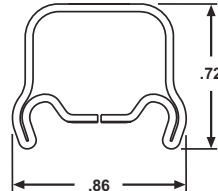
PMR7 Internal Area = 0.298 Sq. In.
