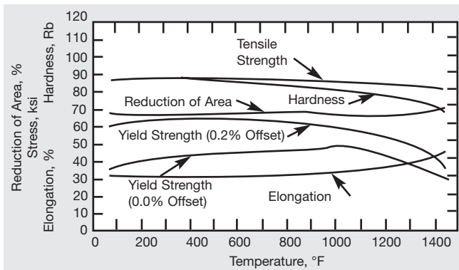
Figure 14. Effect of annealing (3 hr) on room-temperature properties of hot-rolled MONEL alloy 400 plate. At 1470°F, material is fully annealed. (Hardness converted from BHN.).
