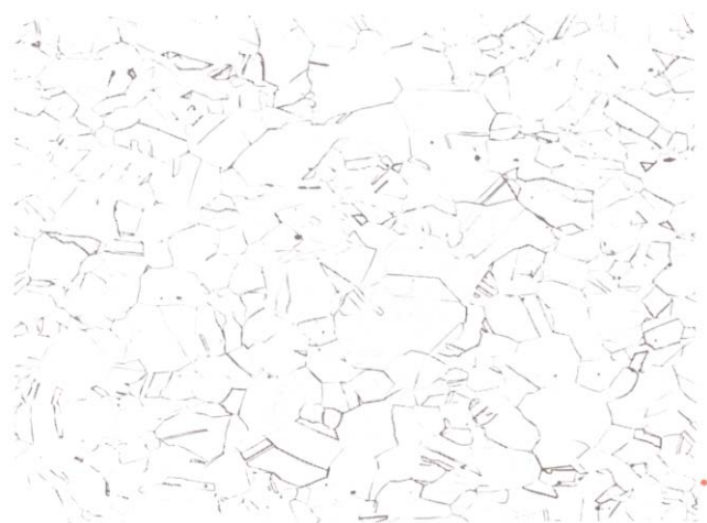
Figure 12. Longitudinal section of cold-drawn MONEL alloy 400 rod. Etchant: Sodium cyanide--ammonium persulfate. 100X.
