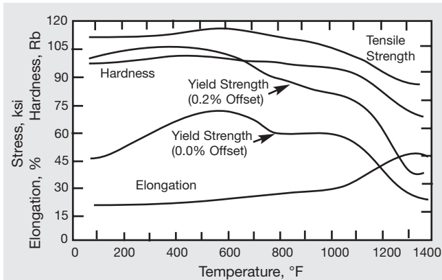
Figure 13. Effect of annealing (3 hr) on room-temperature properties of MONEL alloy 400 cold-drawn rod.
