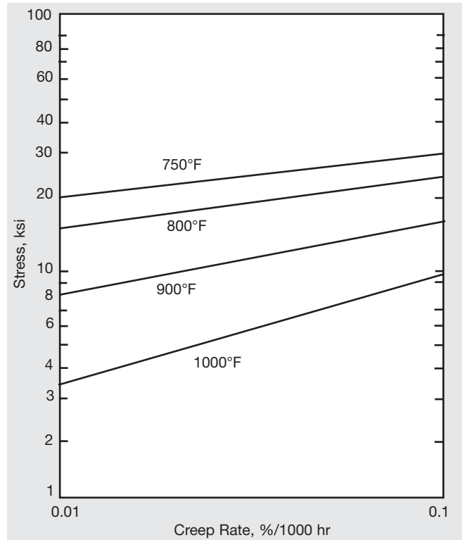
Figure 8. Creep properties of cold-drawn annealed (1500°F/3 hr) MONEL alloy 400.
