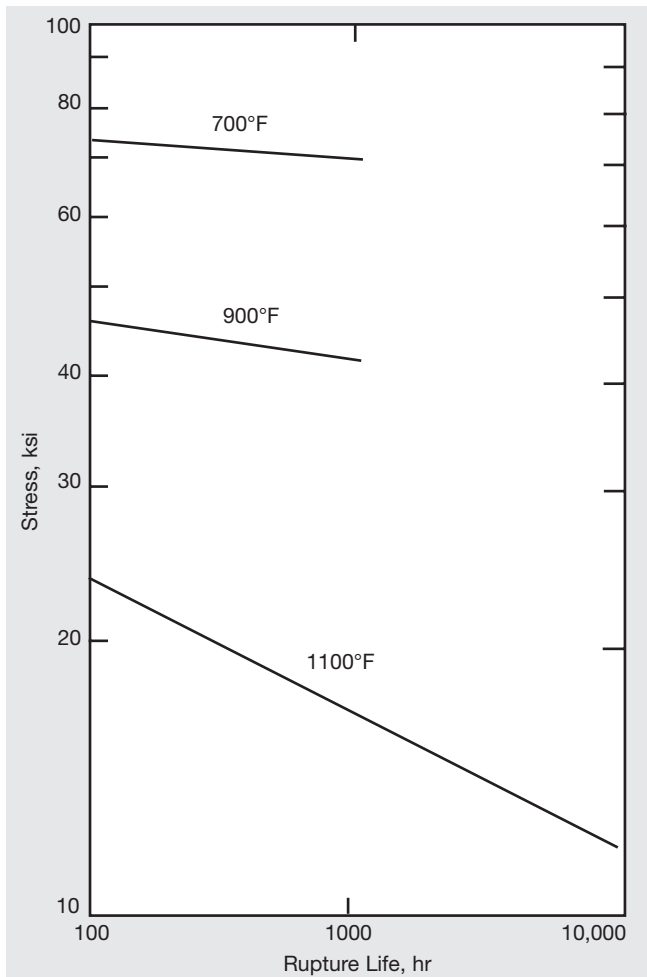
Figure 10. Rupture properties of cold-drawn annealed (1500°F/30 min) MONEL alloy 400.
