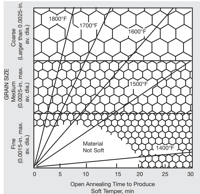
Figure 16. Approximate time required at various temperatures to produce different grain sizes in MONEL alloy 400 cold-rolled strip by open annealing.
