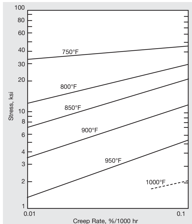
Figure 9. Creep properties of 20% cold-drawn stress-relieved (1000°F/8 hr) MONEL alloy 400.
