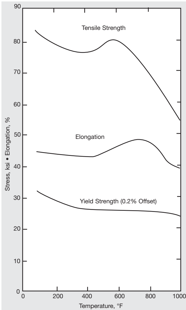
Figure 4. High-temperature properties of annealed MONEL alloy 400.
