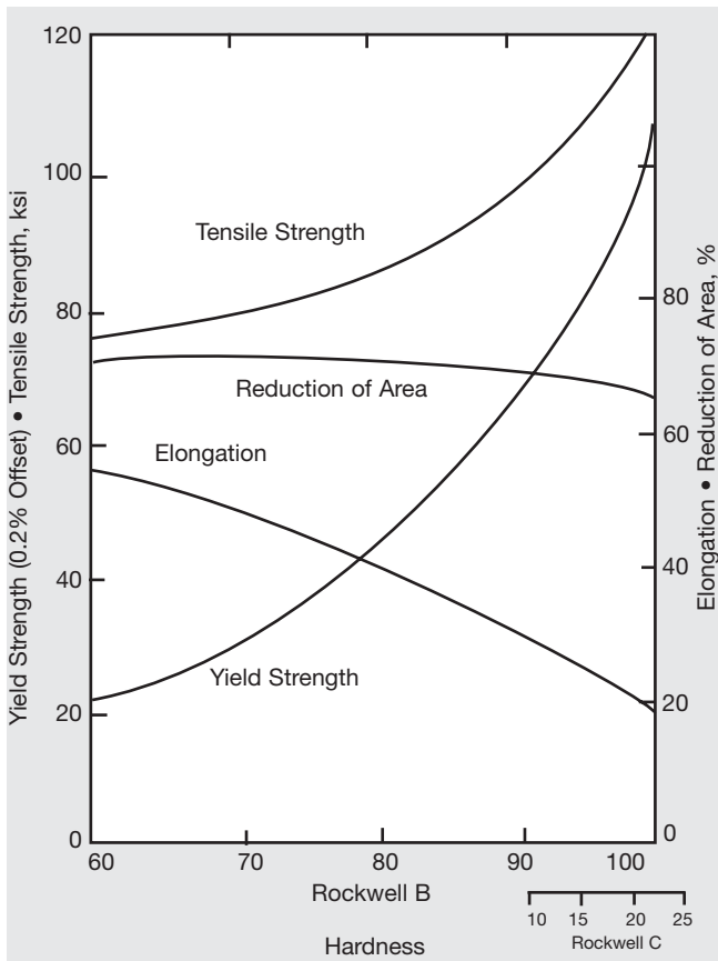
Figure 2. Approximate relationships between tensile properties and hardness of hot-rolled and cold-drawn MONEL alloy 400 rods and forgings.
