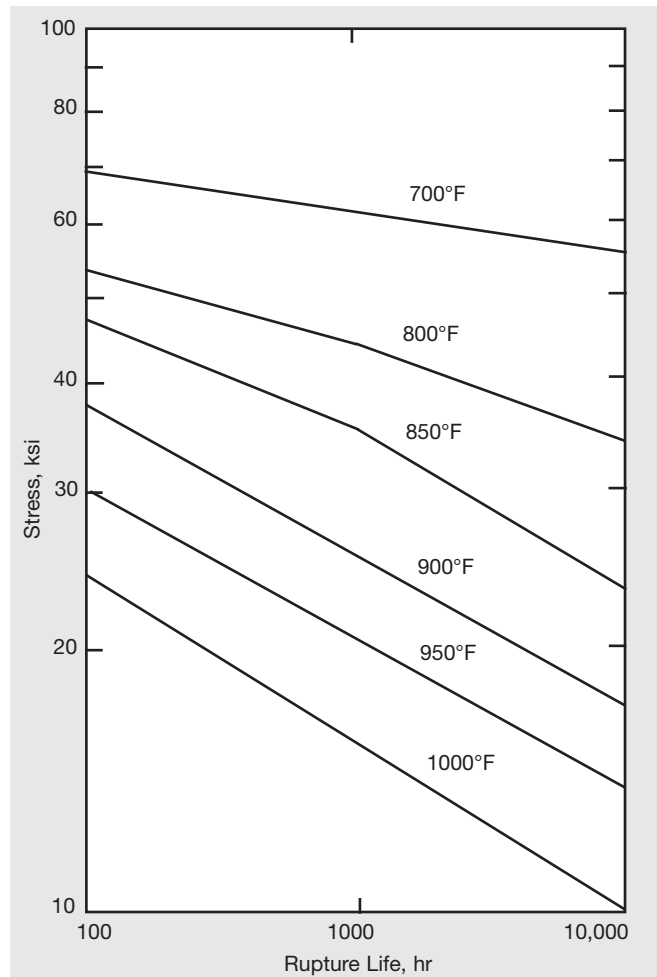
Figure 11. Rupture properties of cold-drawn, stress-relieved (1100°F/8 hr) MONEL alloy 400.
