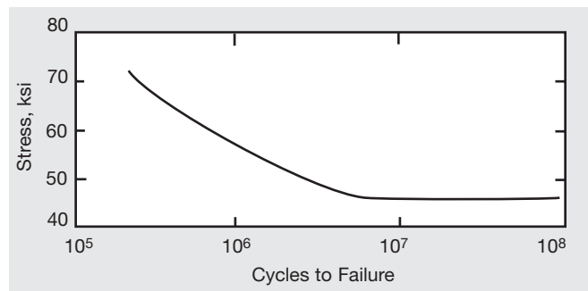
Figure 5. Fatigue strength of commercially produced MONEL alloy 400 wire (0.0375-in. diameter, cold-drawn 75% after final anneal). Tested in processed condition. Data determined with a rotating-wire (5000 rpm) arc-fatigue machine.
