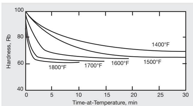
Figure 15. Approximate time required at various temperatures to produce different hardness levels in MONEL alloy 400 cold-rolled strip by open annealing.
