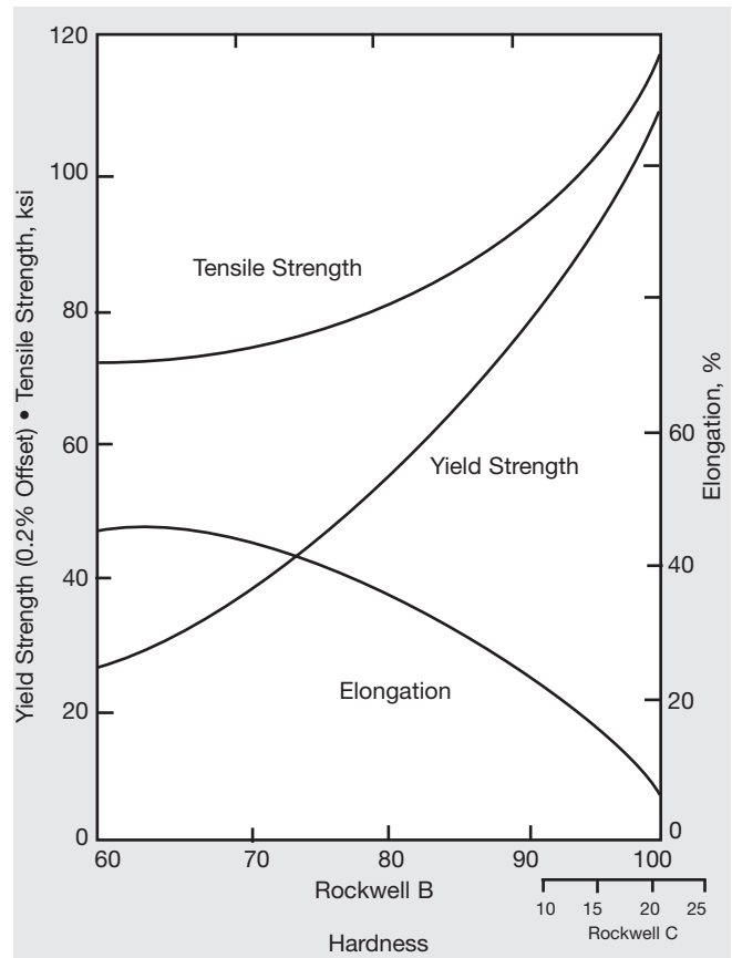
Figure 3. Approximate relationships between tensile properties and hardness of MONEL alloy 400 sheet and strip.
