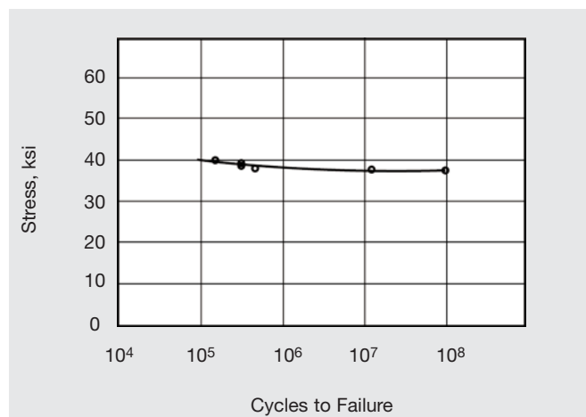
Figure 6. Fatigue strength of commercially produced MONEL alloy 400 rod (0.500-in. diameter, cold-drawn, annealed 1500°F/3 hrs). Tested in the processed condition. Data determined by the R.R. Moore rotating beam technique.
