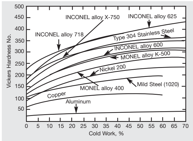
Figure 17. Effect of cold work on hardness.
