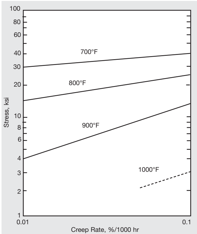
Figure 7. Creep properties of hot-rolled MONEL alloy 400.
