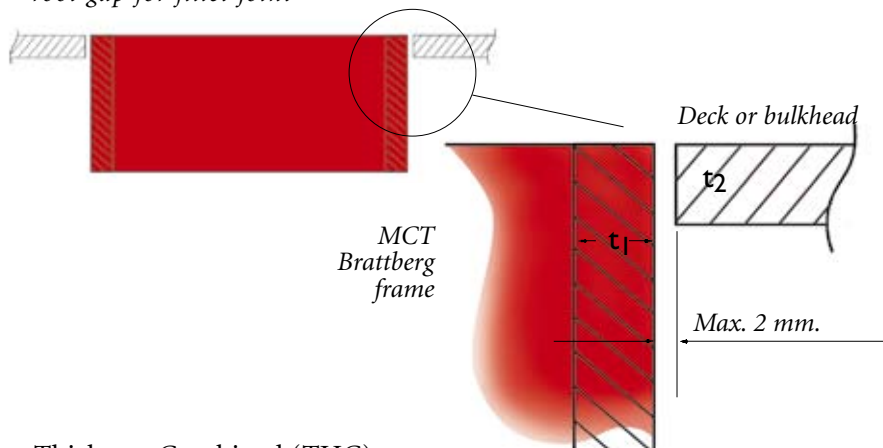
FIG 1: maximum allowable root gap for fillet joint
