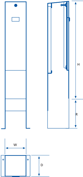
MPA Pillar Height 900mm Width 150mm Depth 160mm
