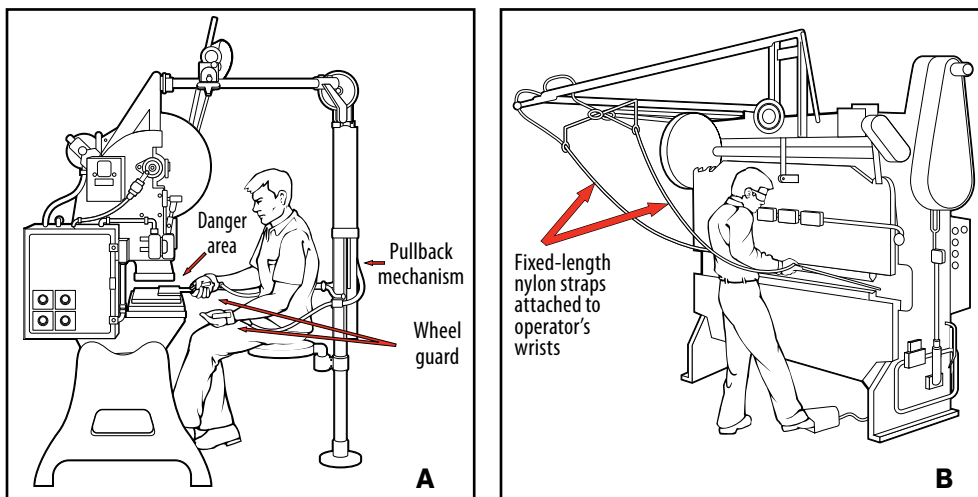
Figure 3.10. Pullback and restraint devices (not in common use). (A) Press operator using pullback devices. The operator's hands are pulled away by cables if the operator leaves them in the danger area. (B) Brake press operator using fixed restraint devices. The operator's hands cannot reach the danger area; hand tools would be required for access.
