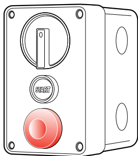
E-stop with run button and main power disconnect
