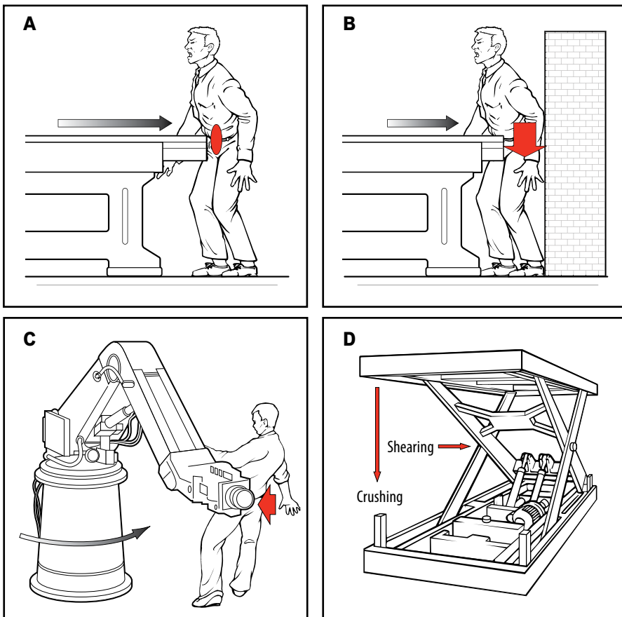
Figure 1.4. Sliding/pivoting movement creating struck by/crushing hazards.
