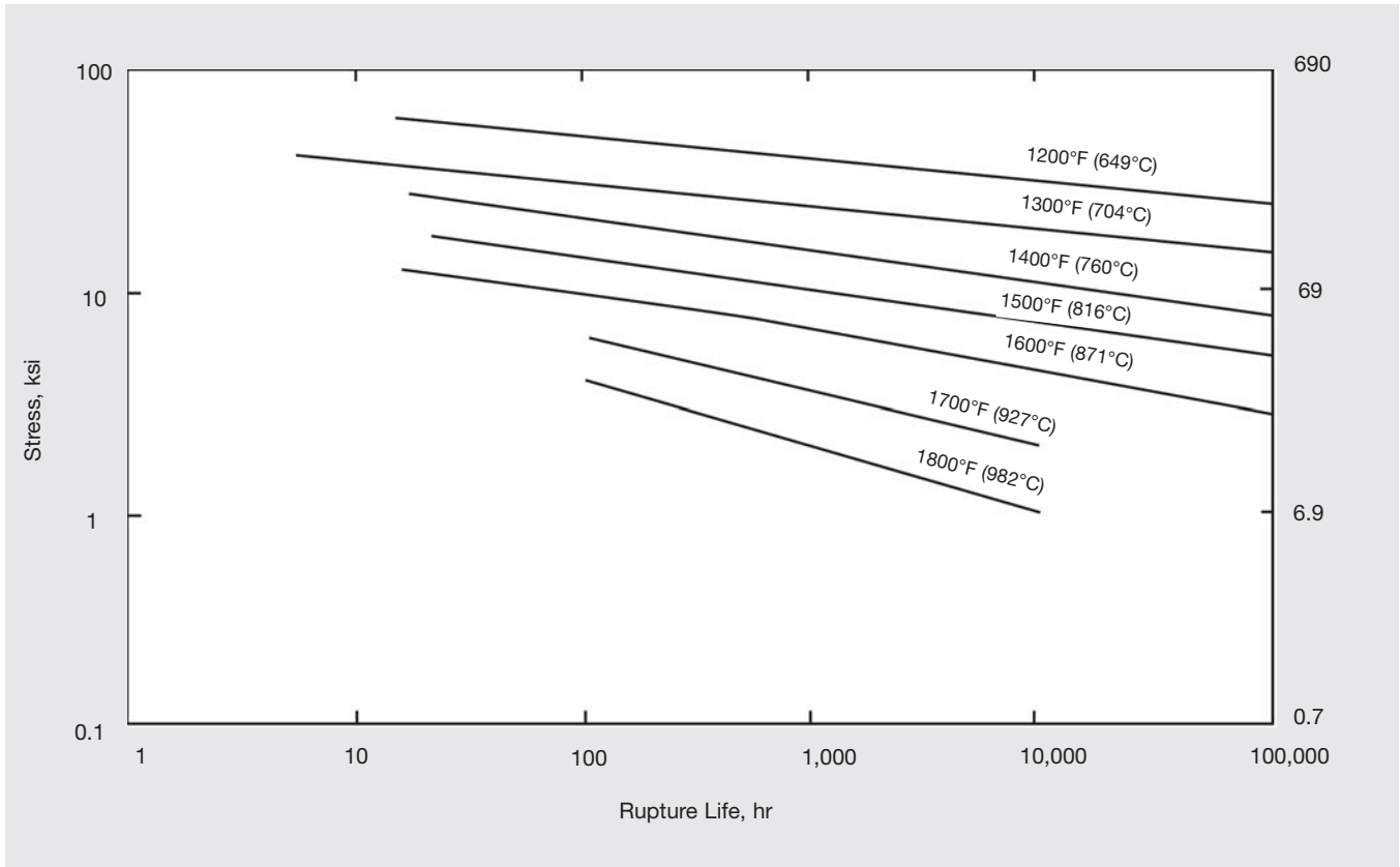
Figure 22. Rupture strength of INCONEL Welding Electrode 112 all-weld metal.
