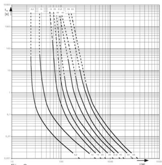
Fig.8 20/36 kV
