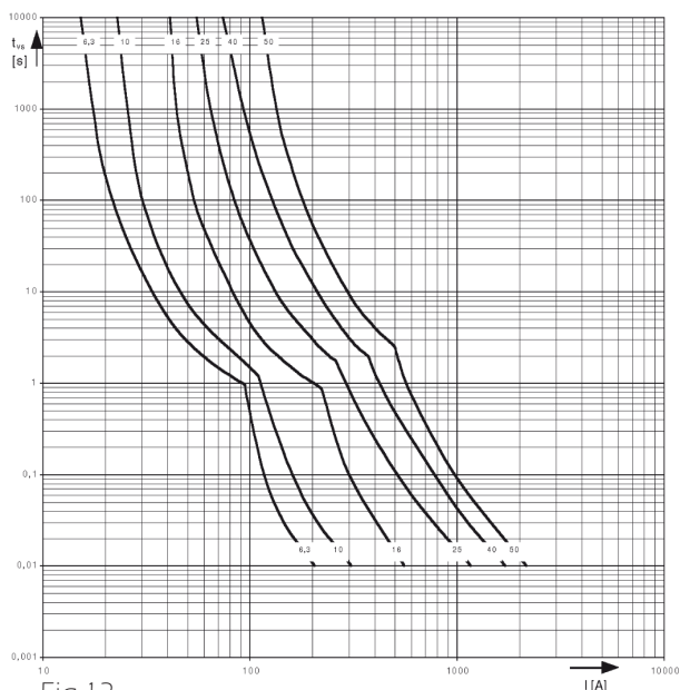
Fig.13 6/12 kV
