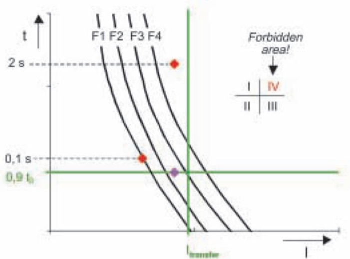
Fig. 11 : Selection of HV fuse-links acc. to VDE 0671 T105
