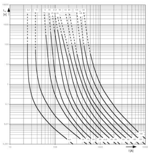
Fig.5 6/12 kV
