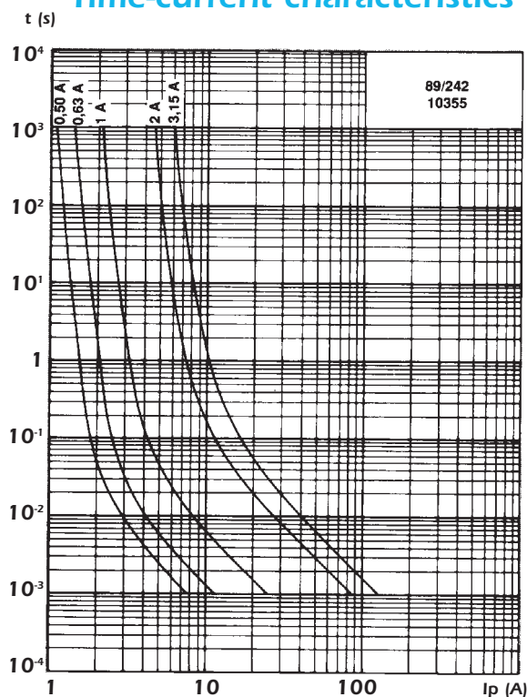
Time-current characteristics
