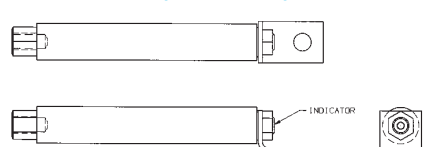
TYPE 30 - EXTERNAL FEMALE TO BOLT (L BRACKET)
