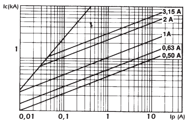
Cut-off characteristics
