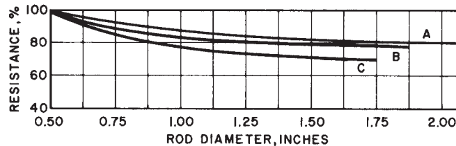
Fig. 11: Diameter of a rod has little effect on its earth resistance Curve A, from Ref. 19 Curve B, average of Underwriters Laboratories tests at Chicago Curve C, average of Underwriters Laboratories tests at Pittsburgh
