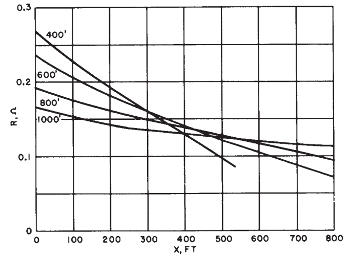
Fig. 30: Intersection curves for Fig. 29. The center of the triangle formed by the intersection, Fig 30 gives the earth resistance 0.146 Ω
