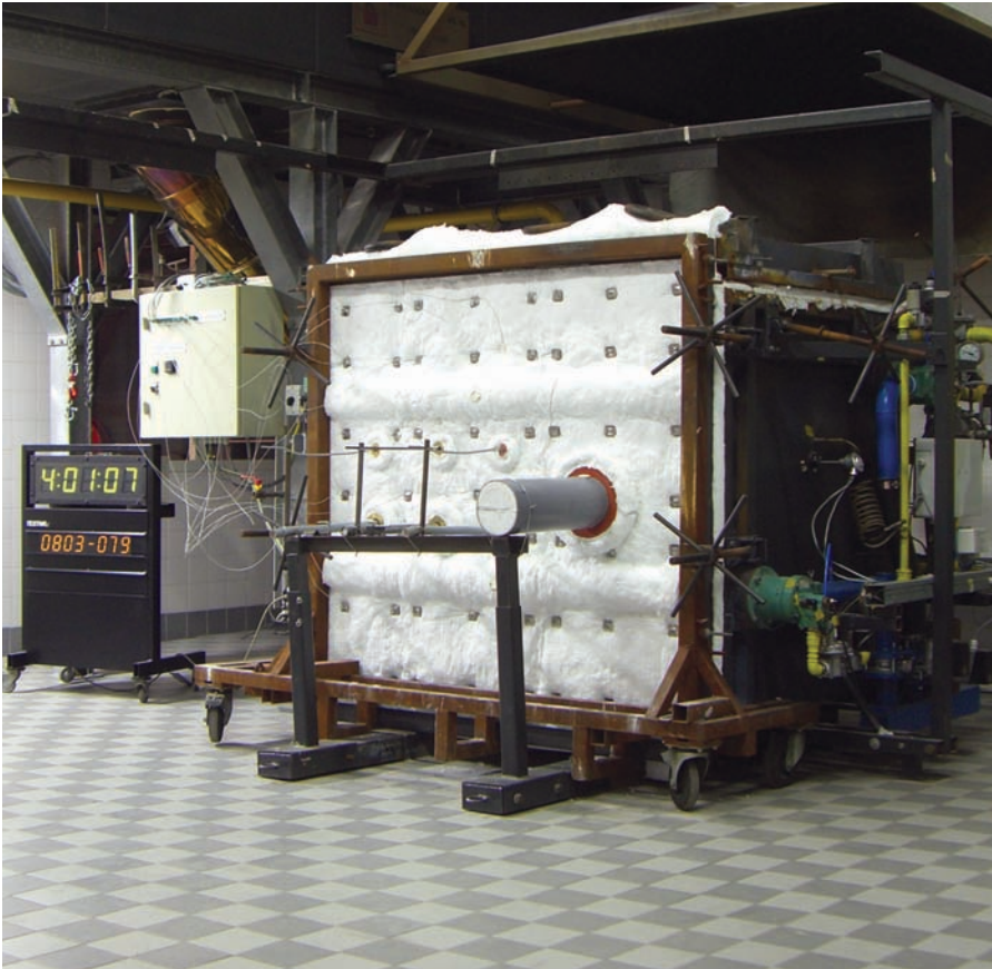
In-house fire testing and pressure testing at CSD International's Laboratories.
