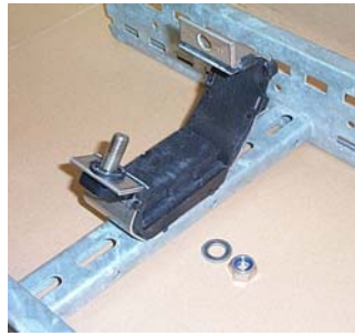
Trefoil Cable
