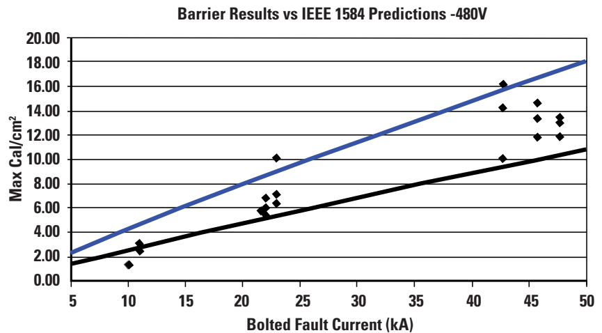
Chart I. Comparison of barrier results to predictions of IEEE 1584 equations for switchgear. The black line represents prediction; the blue line is 167% of the prediction.
