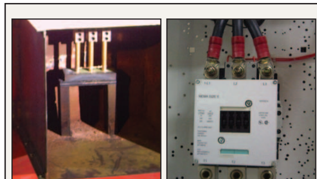
Fig. 2. Barrier test configuration (Left) simulating the line side connections of the starter (Right)
