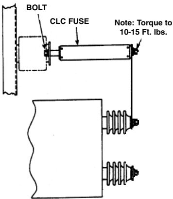
Type CLC Fuse/Capacitor Edgemount on Single Phase Capacitor
